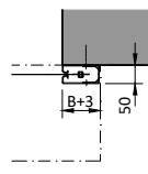
SIDE GUIDE FIXING DETAIL FIXED BETWEEN FACE FIXED
